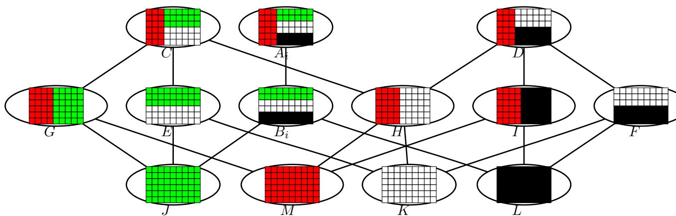
An edge represents a relation Q \prec P if P is above Q . Transitivity edges are not depicted. As an example K \prec E and K \prec C .
