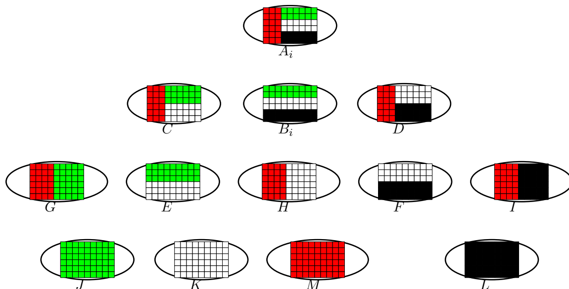
Figure 3: Cantor-Bendixson ranks
